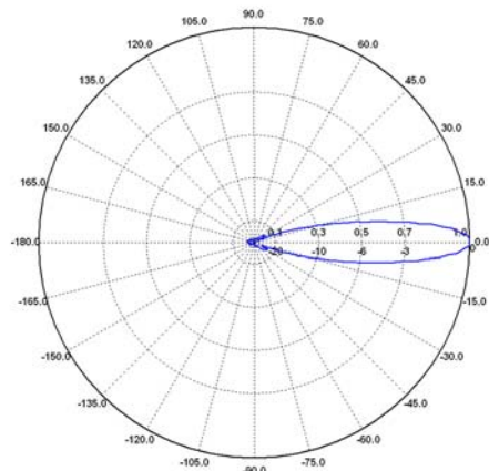
H-Ebene / H-Plane 9 GHz
