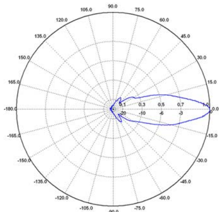
E-Ebene / E-Plane 9 GHz
