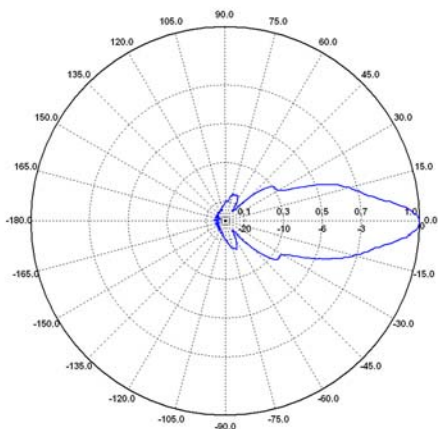
E-Ebene / E-Plane 8 GHz
